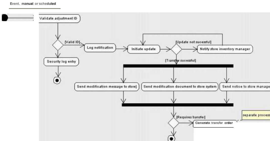
Figure 3.0.2 Adjust Inventory
